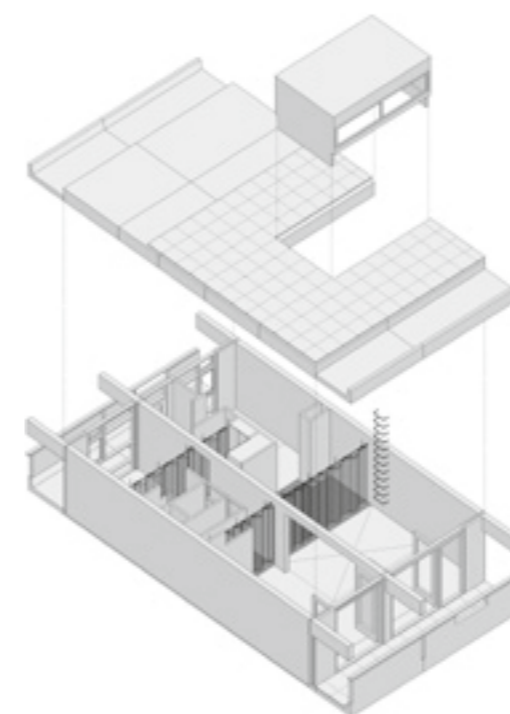
Axonometrie nieuw appartement/ Axonometric projection new apartment
